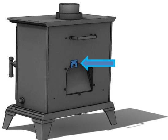
Fig.3 Thermal switch bracket
