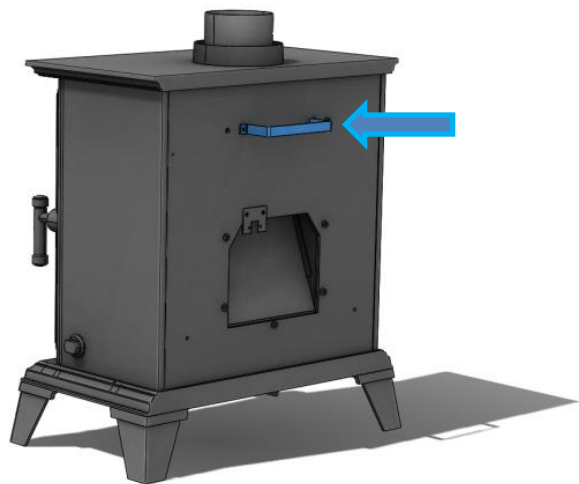
Fig.4 Fitting the thermal switch guard
