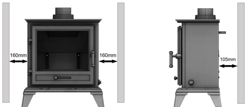
Fig.5 Clearances
